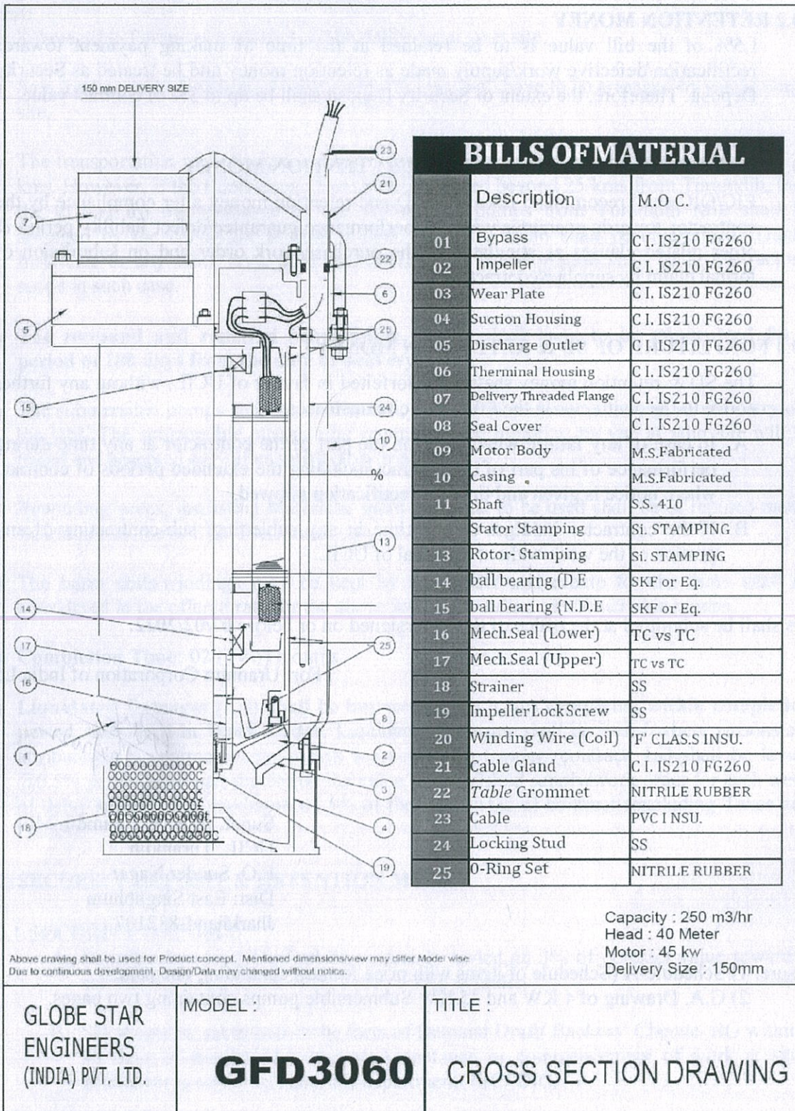
G.A. Drawing of 45 KW Submersible Pump
